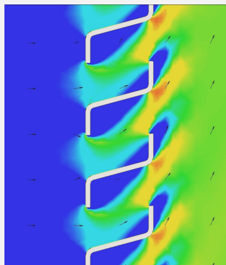
EFD simulation
